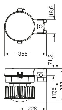
with top mounting module TWM20
