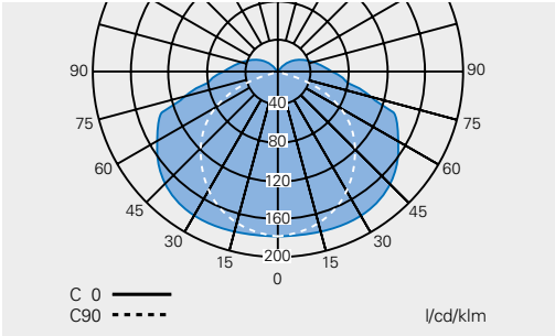
Polar curve nLLK 09018/18 / nLLK 09036/36
